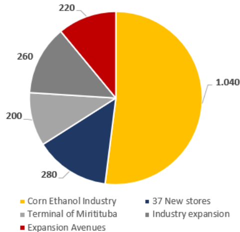
CAPEX breakdown
